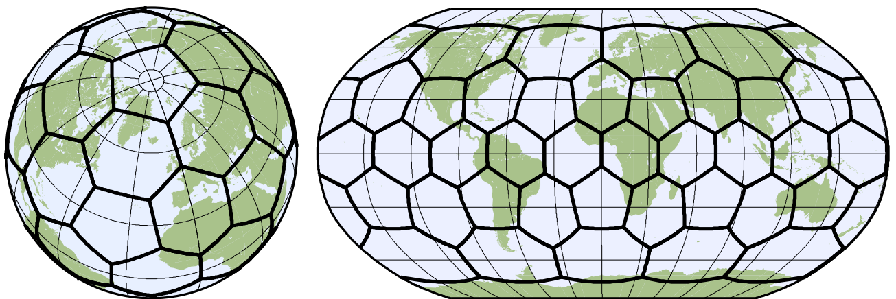
Figure A.2.: Orthographic and Robinson projection of the unstructured grid cells
